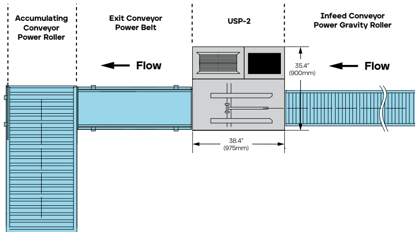
Typical tray feeding & take-away conveyor layout
