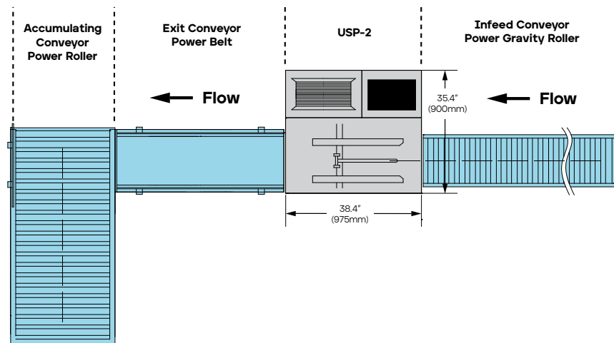
Typical tray feeding & take-away conveyor layout
