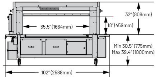
Shown: TRC6-1650 with Standard Conveyor Height See next page for additional track sizes and dimensions.
