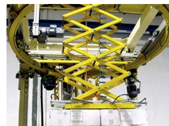
Motorized Hold Down Plate
