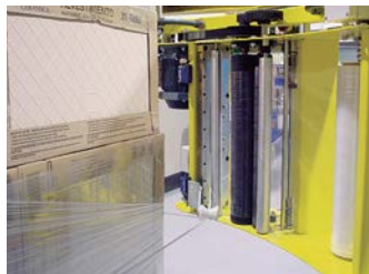
Roping Device
